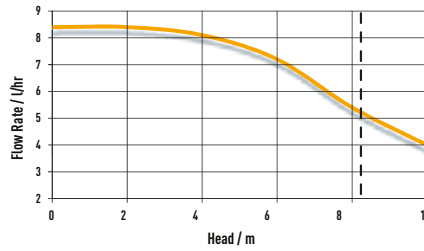
Plot of Flow Rate Against Head
